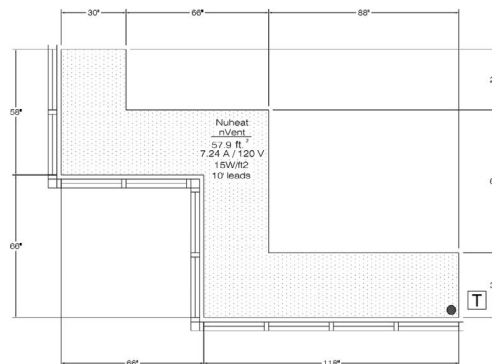
Example of nVent NUHEAT Custom Mat production drawing for a Perimeter Heat application.
