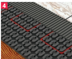
4 Install floor covering covering heated area
